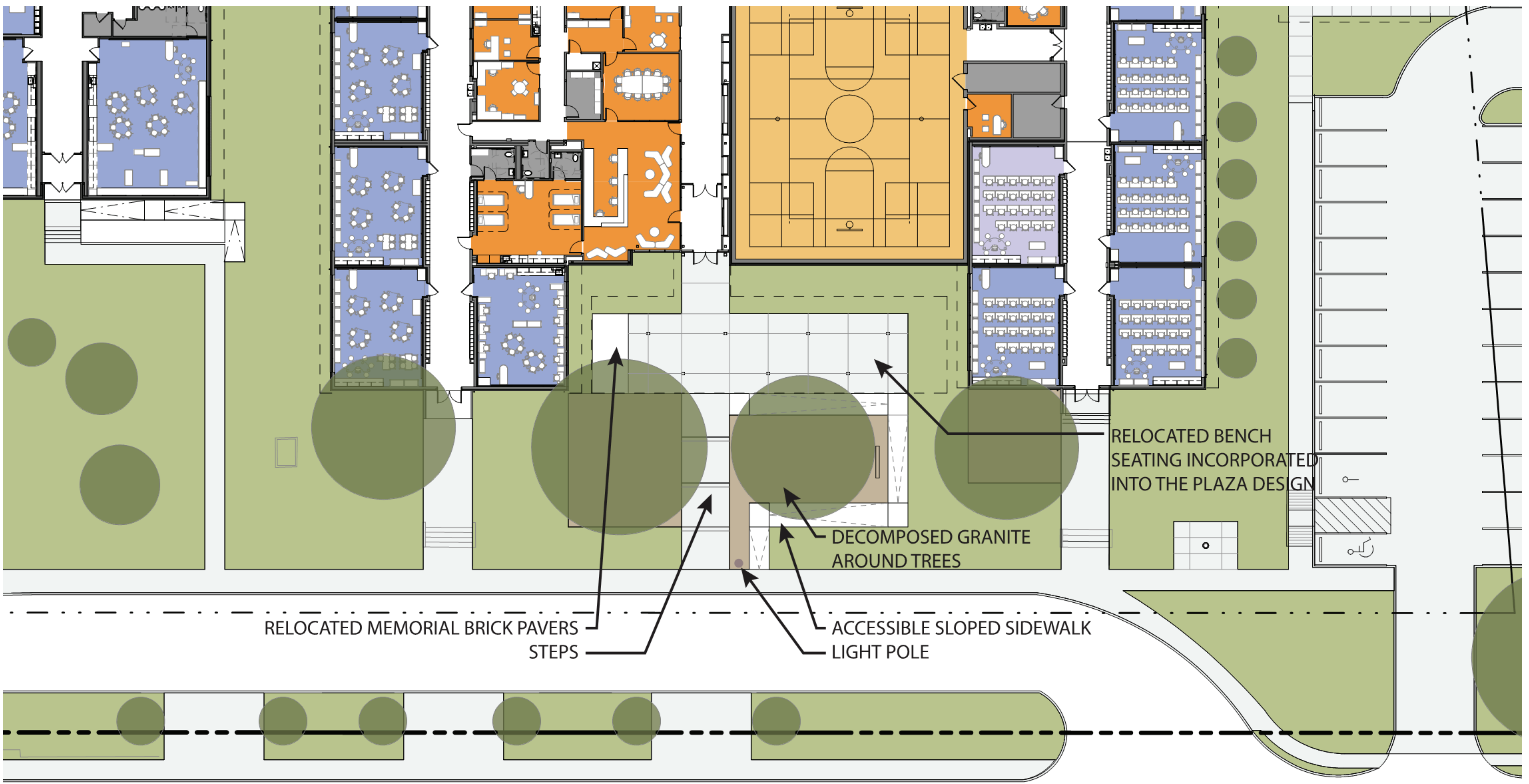
ENLARGED PLAN AT THE FRONT ENTRY
